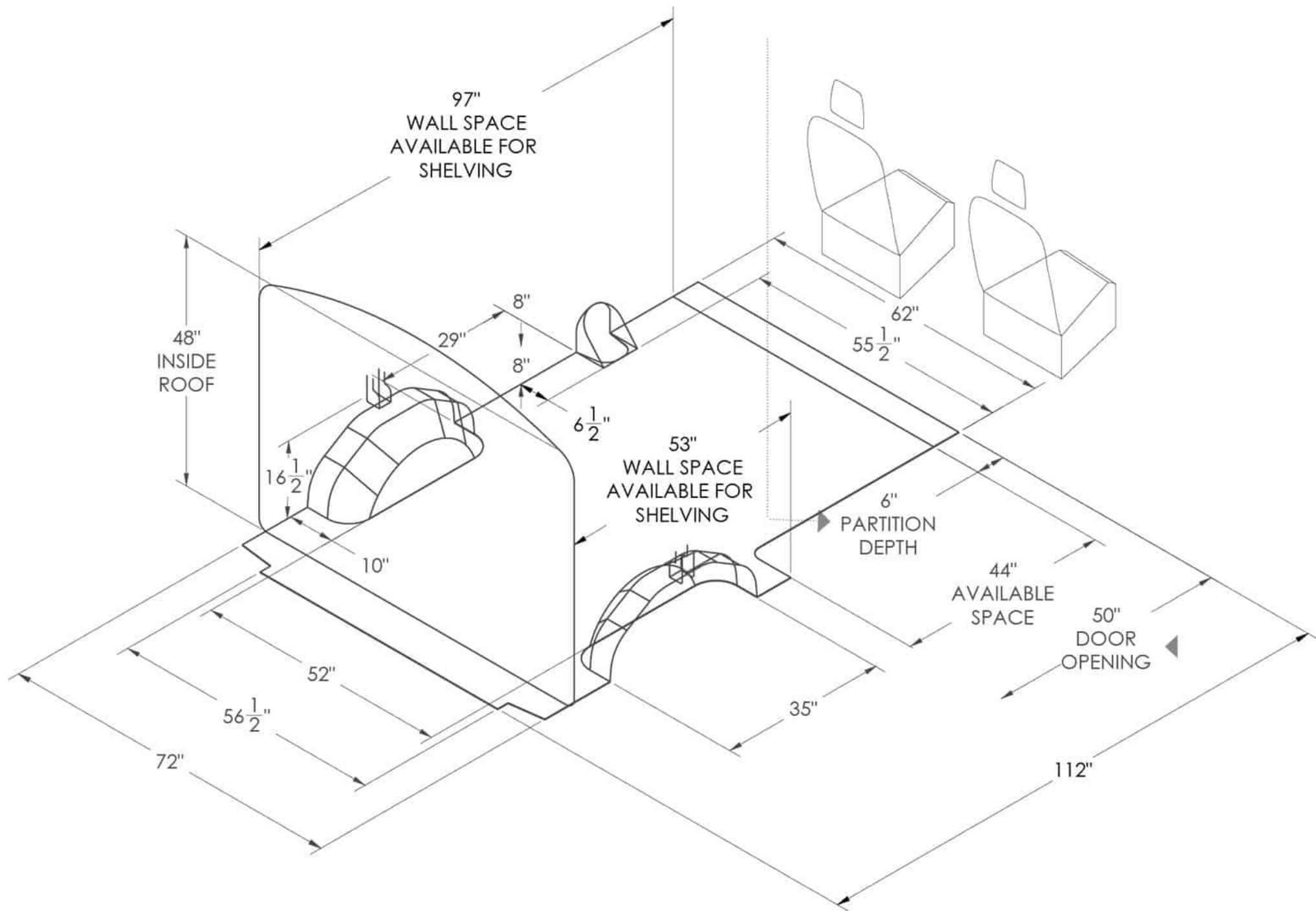
Regular 135" Wheelbase
