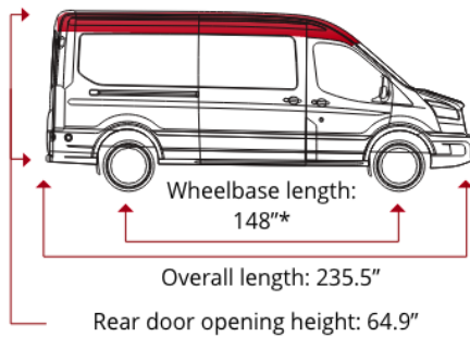
Transit 148 MR
