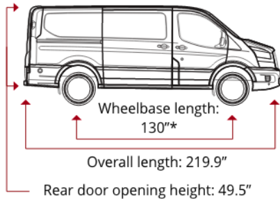
Transit 130 LR
