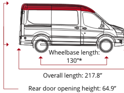
Transit 130 MR
